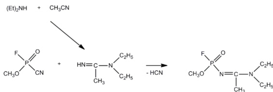
N -[1-(diethylamino)ethyliden]amido- O -methyl-fosforofluoridát
