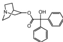
chinuklidin-3-yl-difenyl(hydroxy)acetát, BZ
