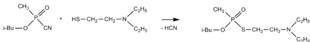
S -[2-(diethylamino)ethyl]- O -isobutyl-methylfosfonothioát
